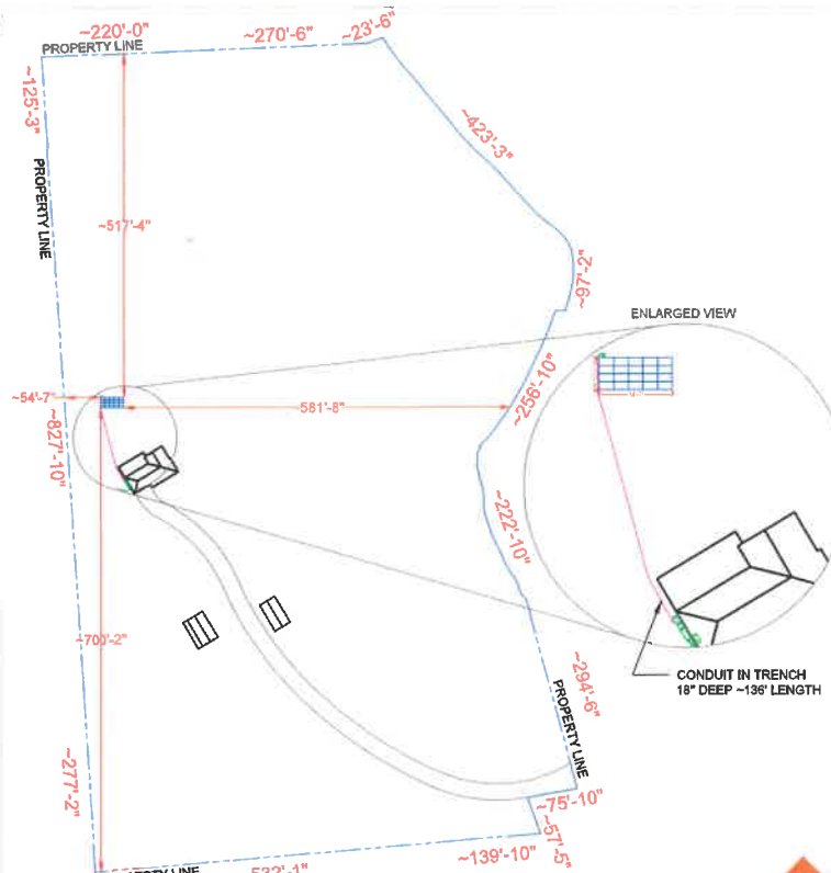
SITE PLAN & SAFETY PLAN SCALE: 1/152" = 1'-0"
