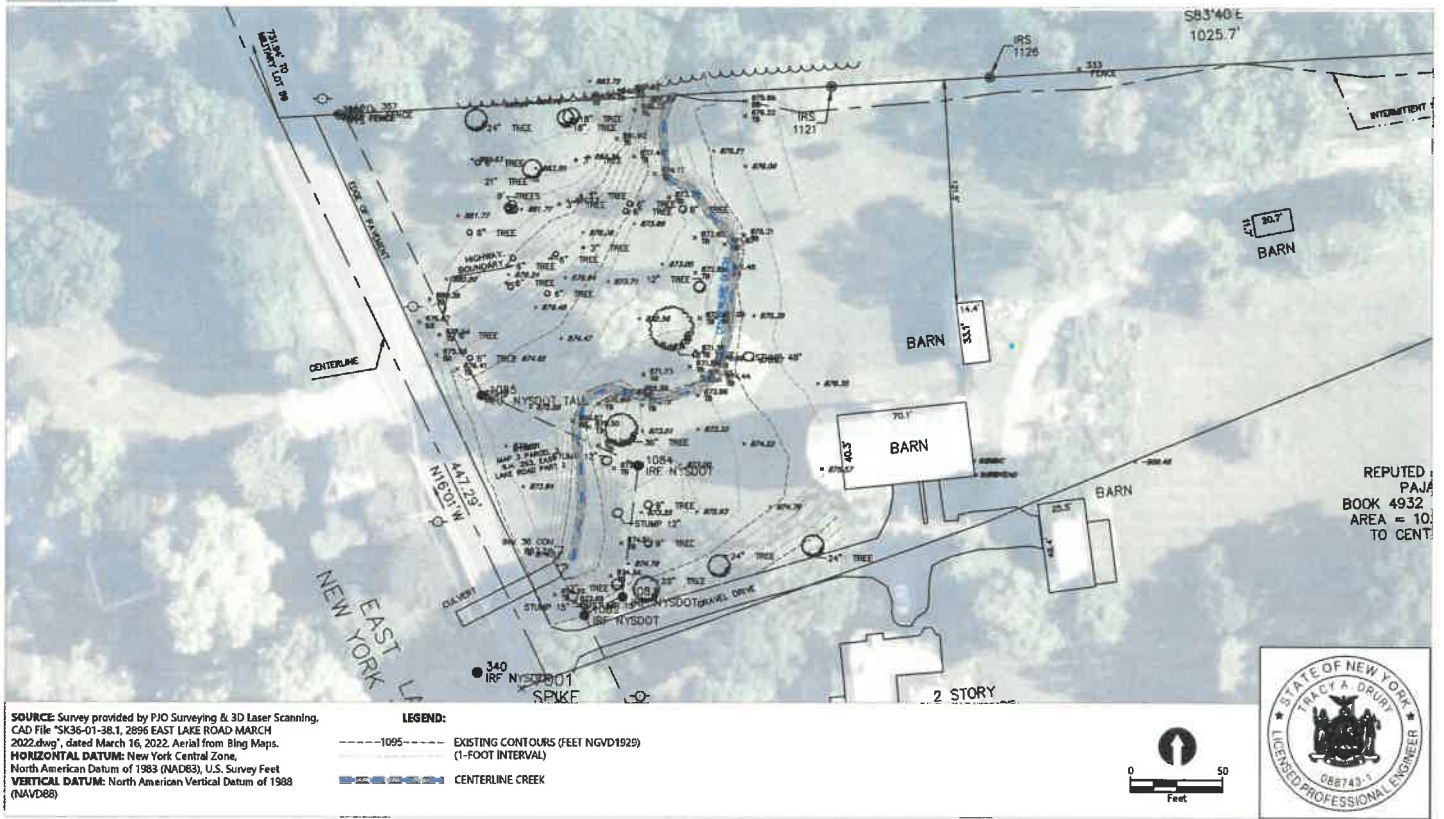
Figure 1b Existing Conditions Pajak Property Skaneateles Lake Association
