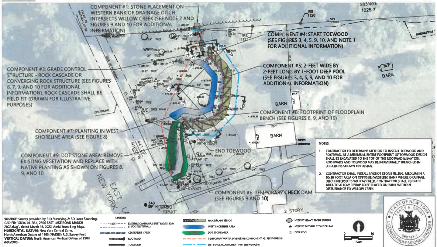
Figure 2 Restoration Plan Pajak Property Skaneateles Lake Association
