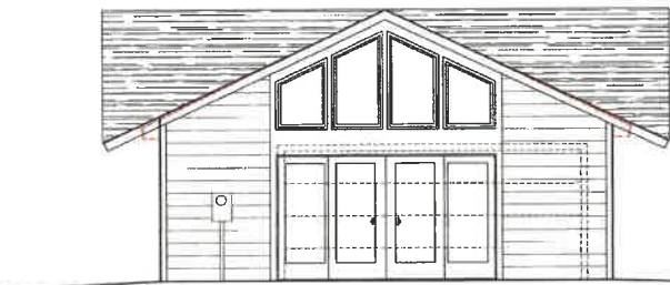
NORTH-WEST ELEVATION 3/16" = 1'-0"
