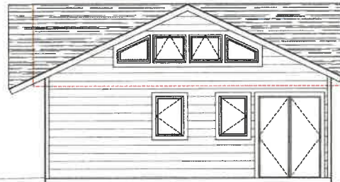
SOUTH-WEST ELEVATION 3/16" = 1'-0"
