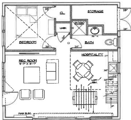
FIRST FLOOR PLAN 3/16" = 1'-0" 589 SF.
